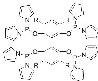
Scheme 2. Ligands used in this study.
